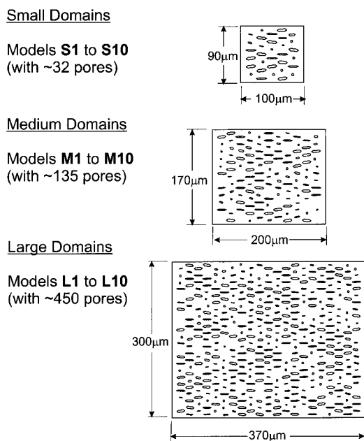
Fig. 4. Illustrations of domains with three different overall sizes (small, medium, large) for \text{Al}_2\text{O}_3 – \text{TiO}_2 coating; for each domain size, 10 separate models were constructed (domains are not drawn in exact proportions).
